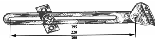
Door stay #33.654.A light duty, 165 mm travel; size 195 mm slot to pivot Door stay #33.654.B light duty, 190 mm travel; size 220 mm slot to pivot Door stay #33.654.C light duty, 270 mm travel; size 300 mm slot to pivot
